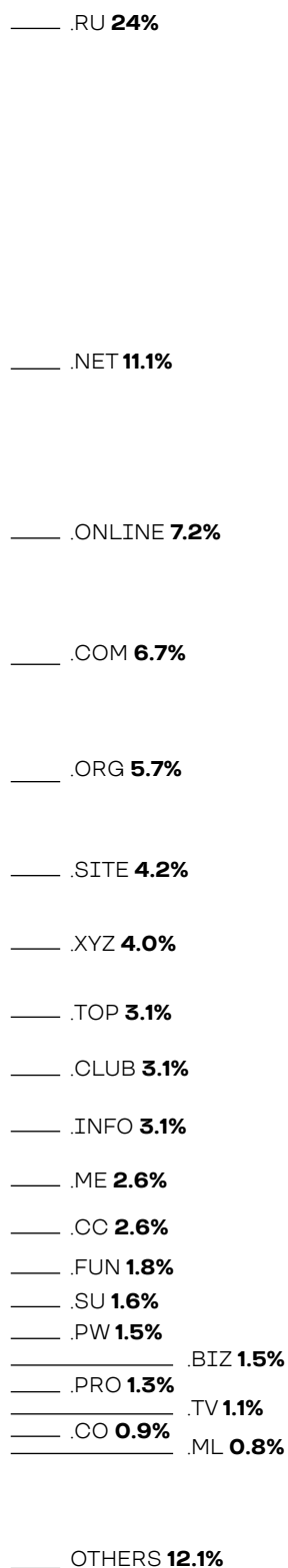
Distribution of dangerous resources by type:
